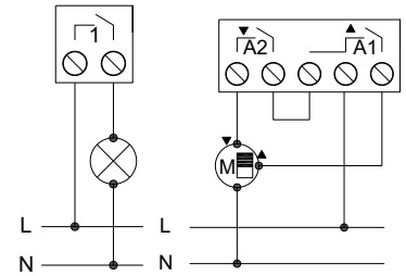
Figure 2: Wiring examples: 1 load and shutter.
