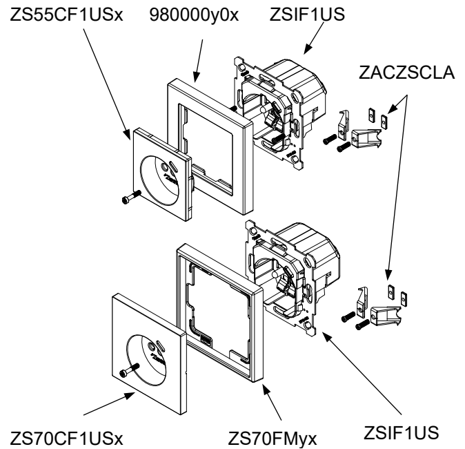
Figure 1. French socket insert with USB C
