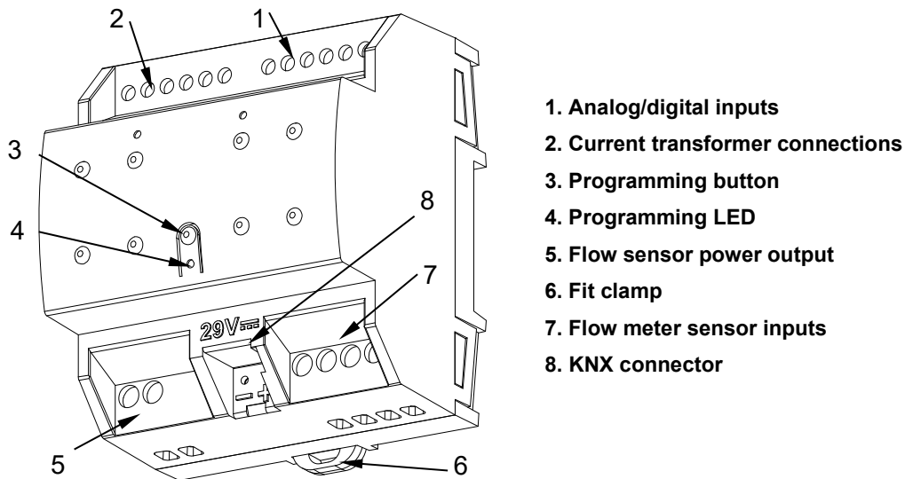
Figure 1. KEM. Element scheme
