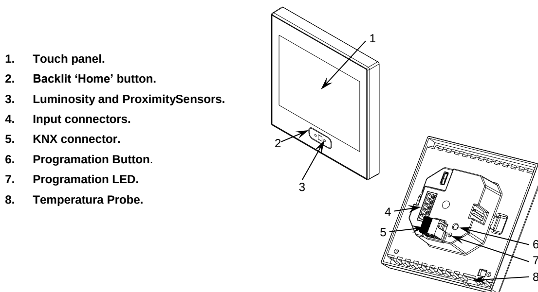
Figure 1. Schematic diagram.
