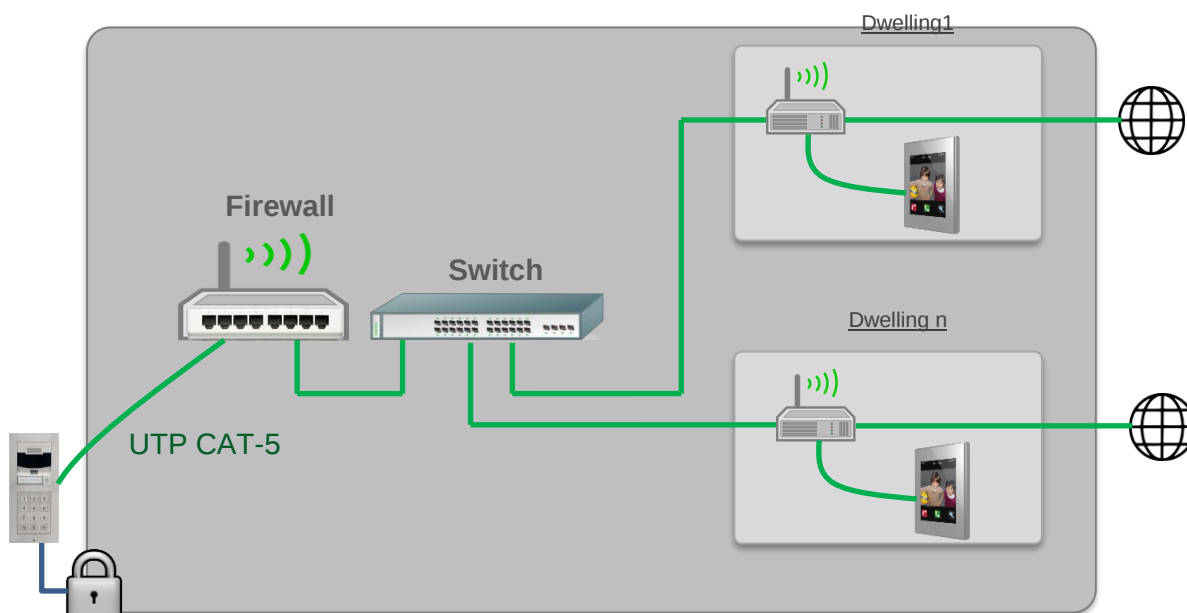
Figure 3 Apartment block installation.
