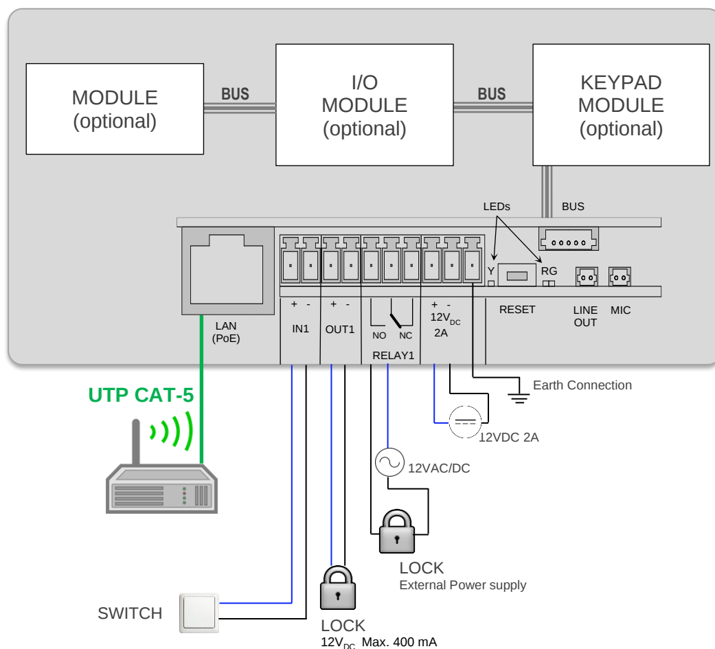
Figure 1 Device wiring diagram.
